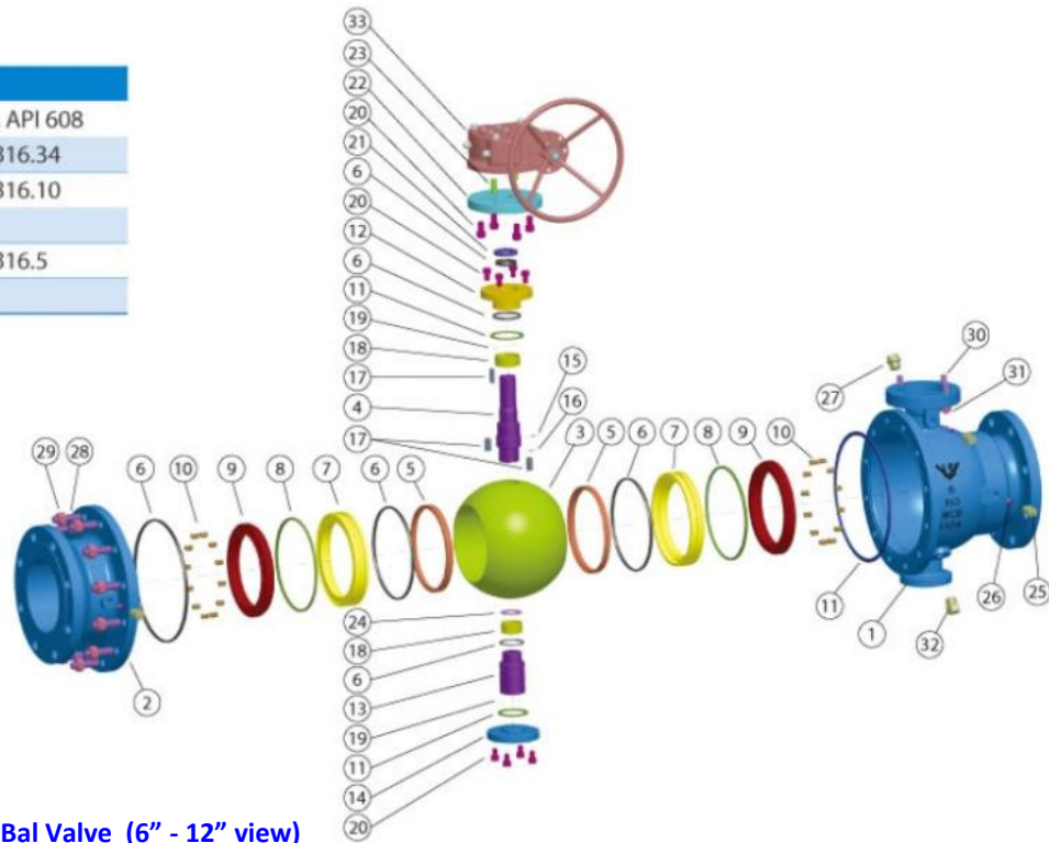
Material List of Trunnion Ball Valve (6" - 12" view)
